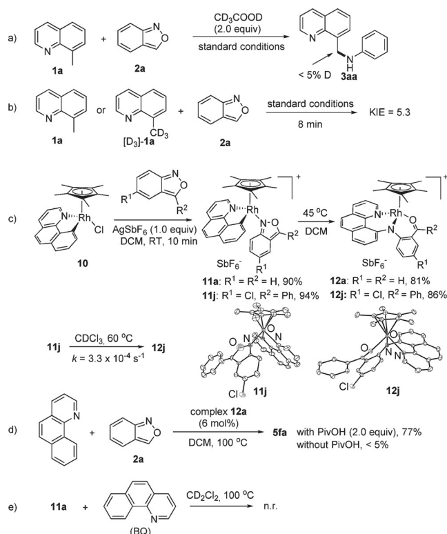
Scheme 6. Mechanistic studies. [24]
