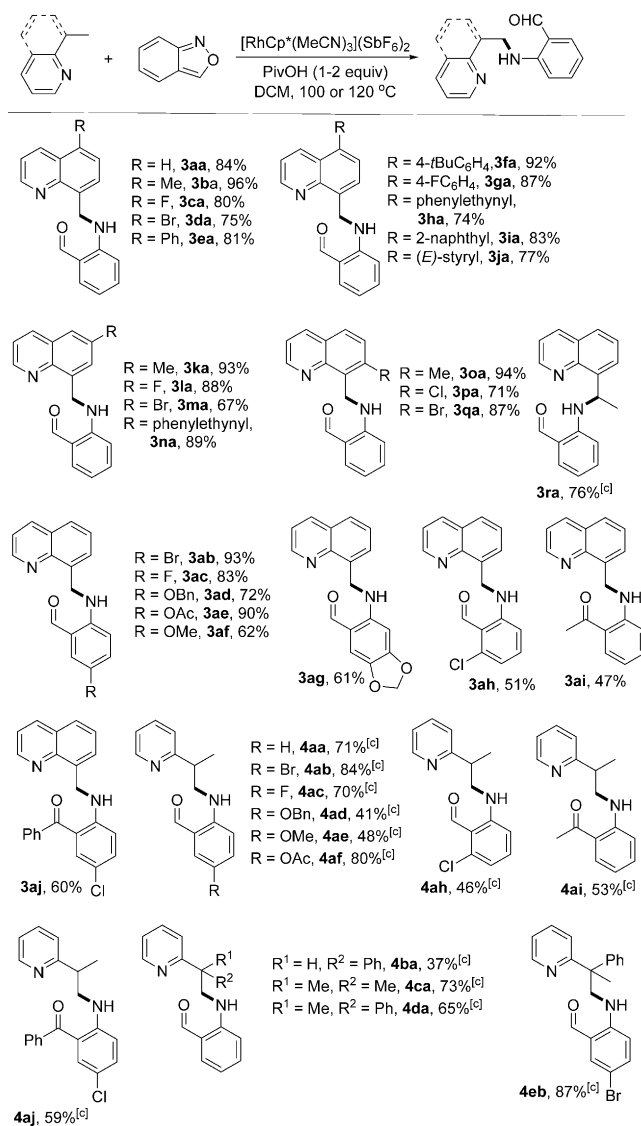
Scheme 2. Amination of C(sp 3 )–H bonds. Reaction conditions: 8-alkylquinoline (0.2 mmol), anthranil (0.4 mmol), [RhCp*(MeCN) 3 ](SbF 6 ) 2 (8 mol %), PivOH (0.2 mmol), DCM (3 mL), 100 °C, 20 h. [b] Yield of product isolated after column chromatography. [c] PivOH (0.4 mmol), 120 °C.
