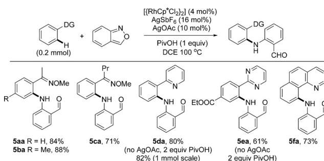
Scheme 3. Amination of arenes (see Supporting Information for details).
