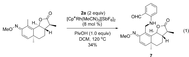
Scheme 3. Amination of arenes (see Supporting Information for details).
